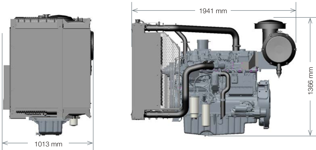
Engine package weights and dimensions
